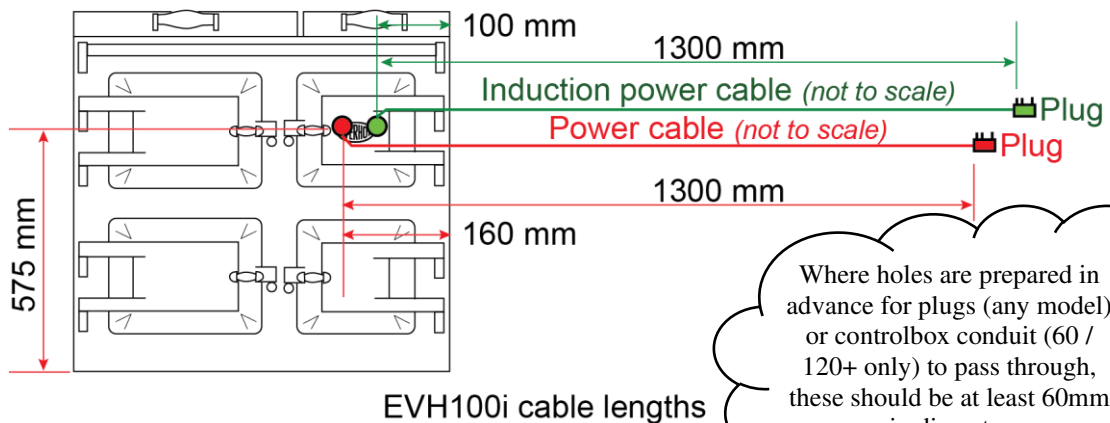
EVH100i dimensions
