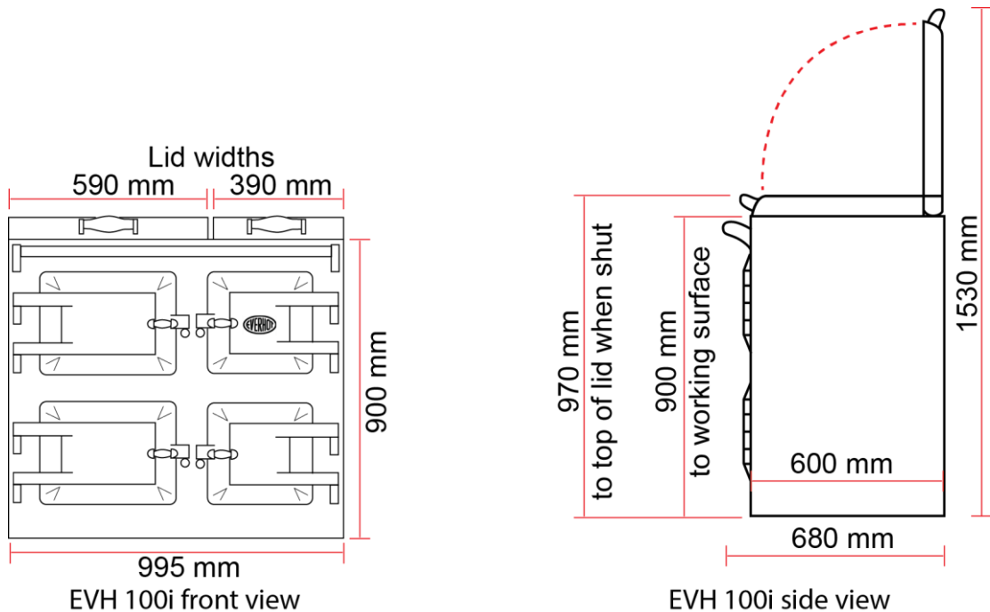
EVH100i dimensions
