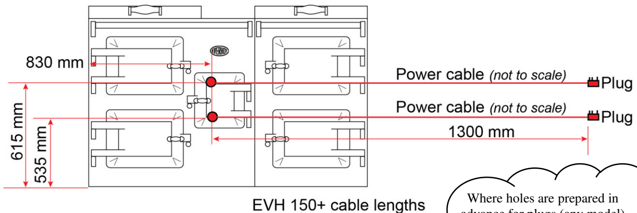
EVH150+ dimensions
