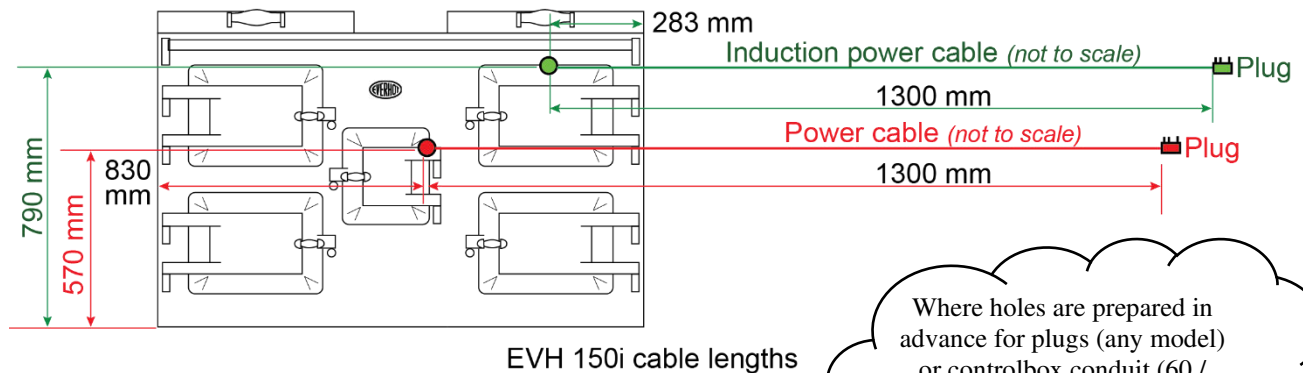
EVH150i dimensions
