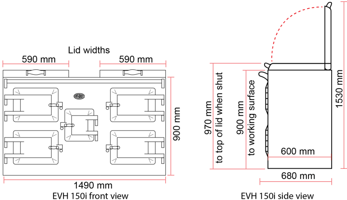
EVH150i dimensions
