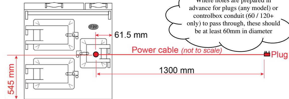
EVH 90+ left-hand oven cable lengths
