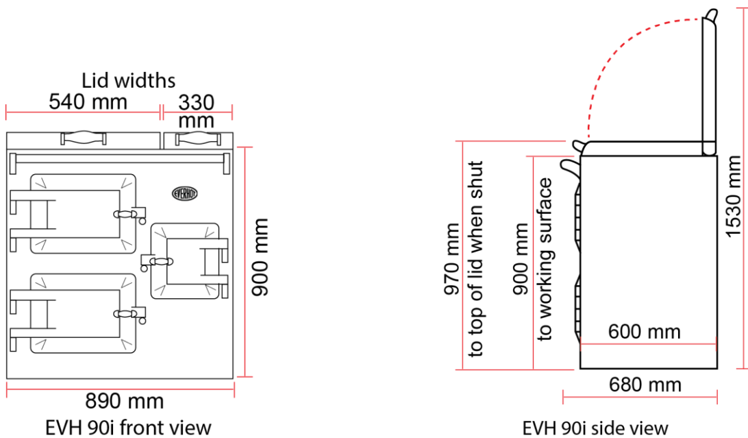
EVH90i dimensions
