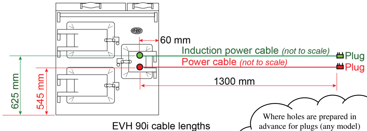
EVH90i dimensions
